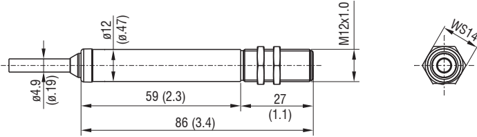
Dimensional drawing thermoMETER FI-SF15-C1, dimensions in mm
