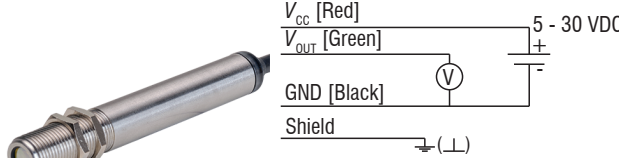
Pin assignment voltage output
