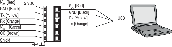
Pin assignment digital output
