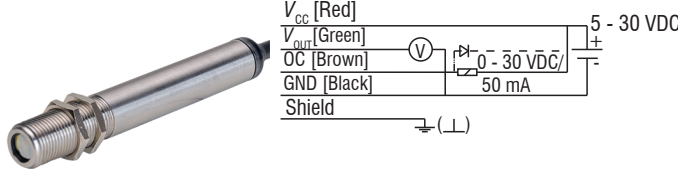
Pin assignment open-collector output
