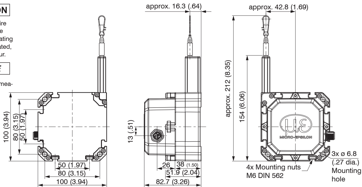
Fig. 5 Dimensional drawing, WPS-3500-K100, WPS-5000-K100, WPS-8000-K100 with 5-pole M12x1 connector, dimensions in mm (inches)
