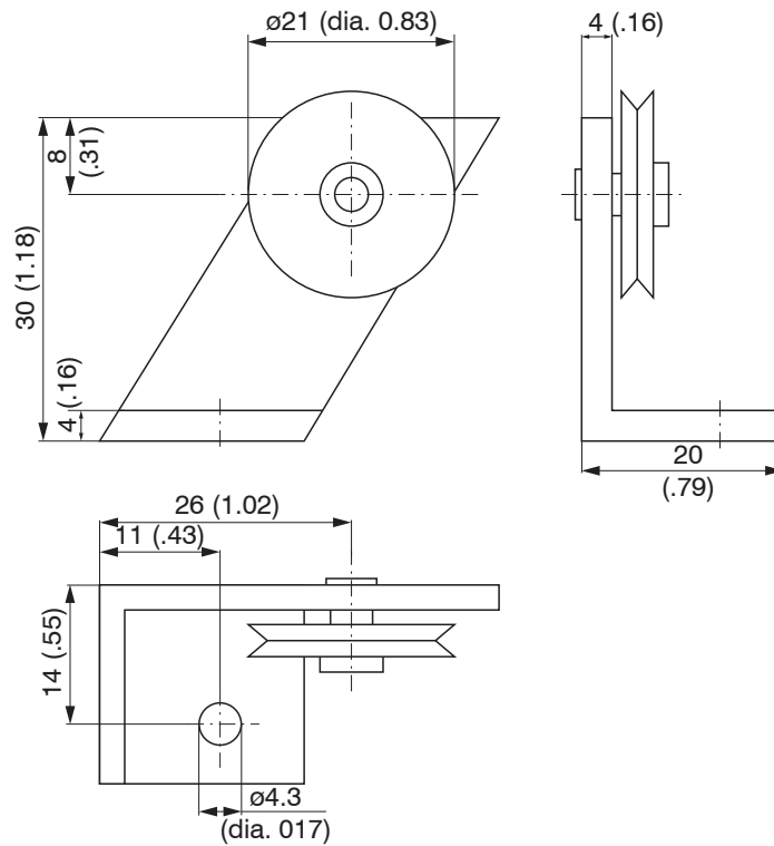
Fig. 14 Deflection pulley TR3-WDS with mounting foot, dimensions in mm
