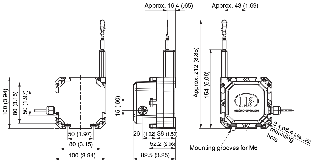
Fig. 3 Dimensional drawing WPS-3500-K100, WPS-5000-K100, WPS-8000-K100 with integrated cable, radial, length 1 m, dimensions in mm (inches)
