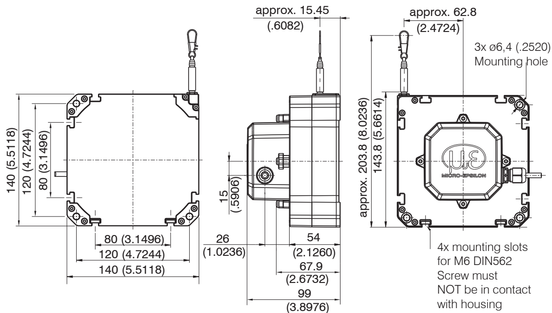
Fig. 6 Dimensional drawing, WPS-12000-K140, with integrated cable, radial, length 1 m dimensions in mm (inches, rounded off)
