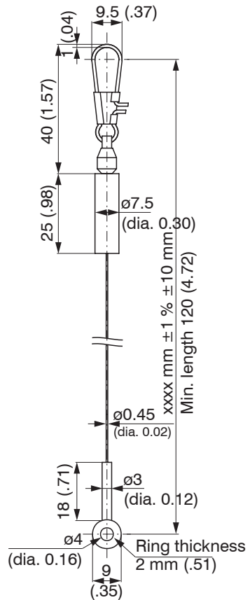
Fig. 15 Wire extension WE-xxxx-CLIP, dimensions in mm
