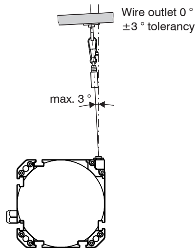
Fig. 7 Attachment and maximum diagonal pull of the measuring wire
