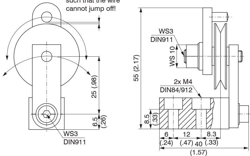
Fig. 13 Deflection pulley TR1-WDS with mounting foot, dimensions in mm
