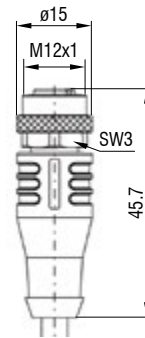
Socket PC5/5
