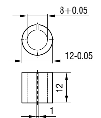
Adapter ring
