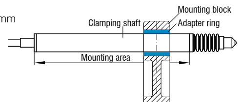
Adapter ring
