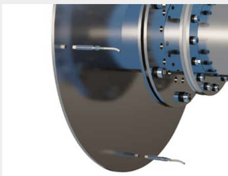
Measuring the radial runout of clutch discs
