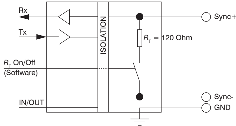
Fig. 16 RS422 synchronization internal circuitry
