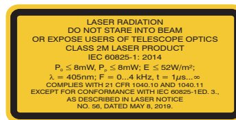
Fig. 2 Laser warning sign and laser label, 29xx-25/BL, 25xx-50/BL, 25xx-100/BL
